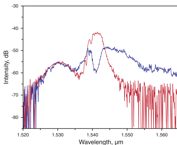
Figure 8 (online color at www.lphys.org ) Optical spectra of the laser radiation during the single-pulse operation mode No. 2: the red line corresponds to the spectrum normally acquired from the output coupler and the blue line – to the spectrum acquired from the FBG
