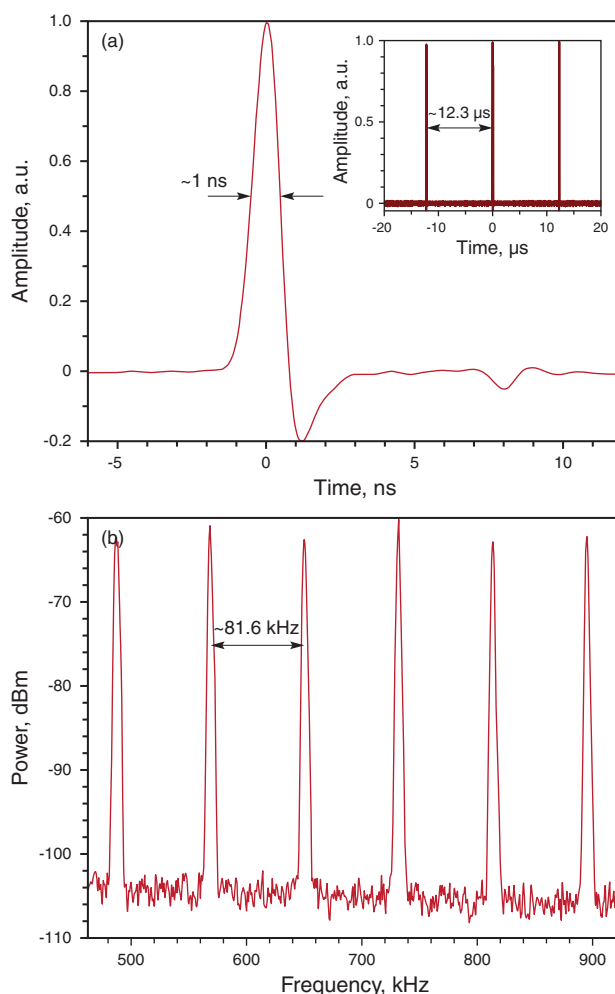
Figure 3 (online color at www.lphys.org ) (a) – oscillograms of the laser output during the single-pulse mode-locked operation (mode No. 1): the red line – high resolution trace of a single pulse; the brown line (inset) – trace of the regular pulse train and (b) – intermode beats spectrum acquired during the single-pulse mode-locked operation (mode No. 1)
