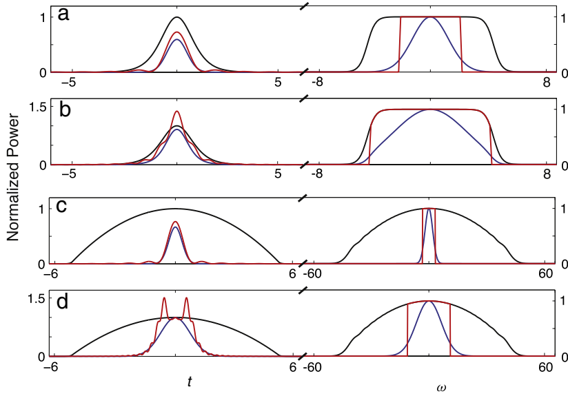
Fig. 25. Normalized temporal and spectral power profiles after the application of a spectral filter. The resultant pulse profiles are obtained from Eq. (94) with a spectral filter of square (red) and Gaussian (blue) shape on initial highly chirped (a, b) hyperbolic secant profile (76) with P = 1 , \tau = 2 , and C = 5 and (c, d) parabolic profile (79) with P = 1 , \tau = 5 , and C = 5 . The spectral filter bandwidth \Omega_F = 4 (a, c), 10 (b, d). (For interpretation of the references to colour in this figure legend, the reader is referred to the web version of this article.)
