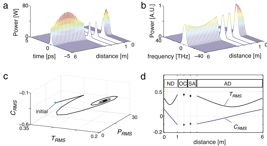
Fig. 28. (a) Temporal and (b) spectral evolution of the power over one round trip once steady state evolution is achieved from the solution to Eqs. (99)–(100) with discrete actions (92) and (93). A doped-fibre with parameters \beta_2 = 0.1 \text{ ps}^2/\text{m} , \gamma = 0.005 \text{ 1/(W m)} , g_0 = 2.76 \text{ 1/m} (corresponding to 12 dB total gain), E_s = 1 \text{ pJ} , \Omega_g = 10 \text{ THz} , and L = 1 \text{ m} is followed by an output coupler with R = 0.9 and a saturable absorber with q_0 = 0.3 \text{ 1/m} and P_s = 3 \text{ W} . The saturable absorber is followed by 5 m of passive fibre with \beta_2 = -0.022 \text{ ps}^2/\text{m} and \gamma = 0.005 \text{ 1/(W m)} . (c) Poincaré map taken at the beginning of the normal dispersion segment. (d) Intra-cavity evolutions of the RMS pulse duration and chirp parameter once steady state evolution is reached.
