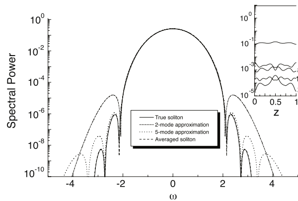
Fig. 11. Spectral power of DM soliton in logarithmic scale: true DM soliton (solid line), solution of path-average Eq. (61) (dashed line), two-mode (dashed–dotted line) and five-mode (dotted line) approximations using a Gauss–Hermite expansion [130]. Inset: dynamics of the first nonzero coefficients in the expansion over one map period.
