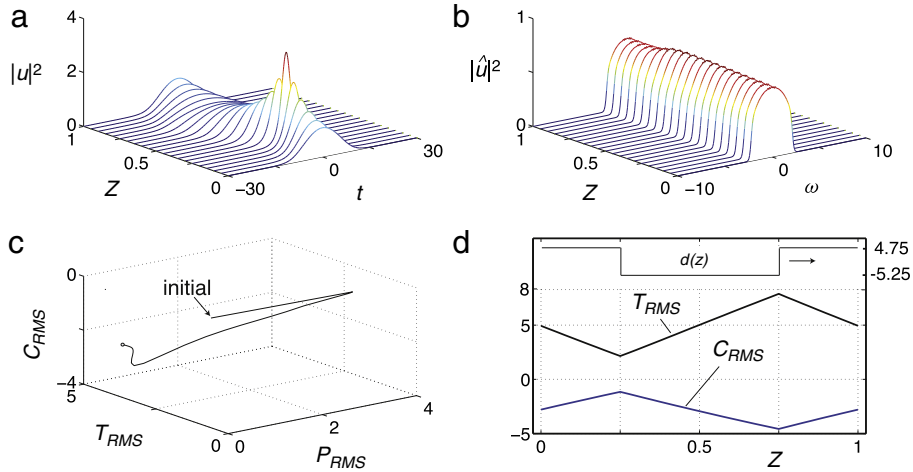
Fig. 19. (a) Temporal and (b) spectral evolution of the power per map period once steady state evolution is achieved from the solution to Eqs. (82)–(84). Here equation parameters are the same as in Fig. 17, but with large net-normal dispersion \bar{d} = -0.25 and gain filtering parameter \nu = 0.1 . (c) Poincaré map taken in the middle of the anomalous dispersion segment. (d) Intra-map evolutions of the RMS pulse duration and chirp parameter once steady state evolution is achieved.
