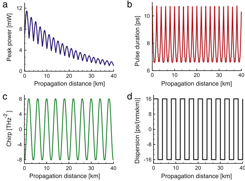
Fig. 12. Evolution of the DM soliton (a) peak power, (b) FWHM pulse duration, and (c) chirp parameter along one section of the transmission system with short-scale dispersion map (shown in (d)). The average dispersion value is \langle D \rangle = 0.1 \text{ ps}/(\text{nm} \times \text{km}) , nonlinear parameter is \gamma = 2.43 \text{ 1}/(\text{W km}) and fibre loss is \alpha = 0.21 \text{ dB/km} . The amplification distance is 40 km and the dispersion compensation length is 4 km.
