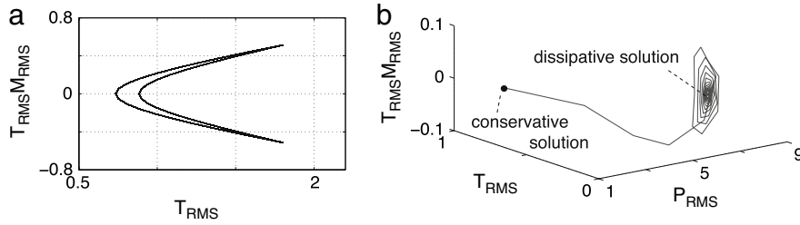
Fig. 5. Visualization of dispersion managed soliton dynamics. (a) Phase plane dynamics showing the evolution of pulse parameters over one dispersion map period for a conservative DM system. (b) Poincaré map showing the stroboscopic long-scale evolution of the pulse parameters at one particular point (shown here in the middle of the anomalous segment) in the dispersion map over many map periods. The examples shown here correspond the conservative case in (a), and a dissipative DM solution whose initial condition is the same as the DM soliton considered in (a). Note the dissipative terms attract the solution to a different point in the phase space.
