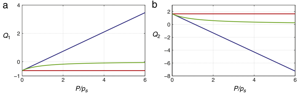
Fig. 20. Nonlinear gain functions (a) Q_1 and (b) Q_2 in Eq. (91) for the cubic GLE where F(x) = 1 (red), the cubic–quintic GLE where F(x) = 1 - x (blue), and a saturable GLE where F(x) = 1/(1 + x) (green). (For interpretation of the references to colour in this figure legend, the reader is referred to the web version of this article.)
