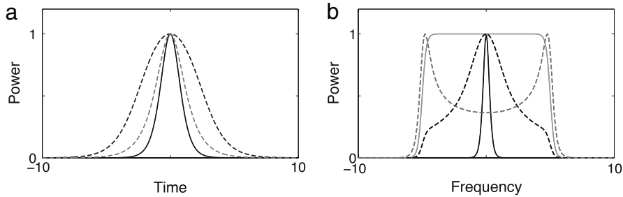
Fig. 15. Hyperbolic secant solutions (76) for P = 1 , \tau = 1 , C = 0 (solid black) and C = 5 (solid grey) in both the (a) temporal and (b) spectral domains. The dashed profiles are examples of highly chirped solutions to the CQGLE [97–101].
