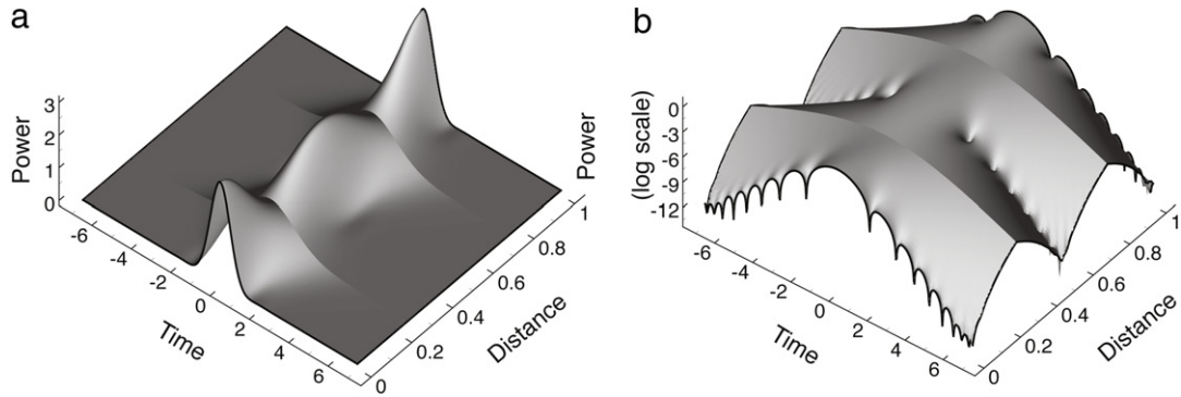
Fig. 6. Breathing dynamics of a DM soliton propagating over one dispersion map period.
