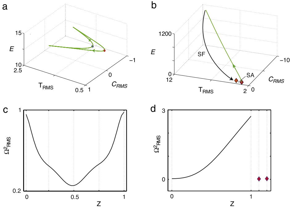
Fig. 27. Pulse RMS quantities energy E , pulse duration T_{RMS} , and chirp parameter C_{RMS} phase plane along with the RMS bandwidth parameter evolution from the data obtained in (a, c) Fig. 17 and (b, d) (a, c) Fig. 26. The RMS parameters are shown over one map period once steady state evolution is obtained.
