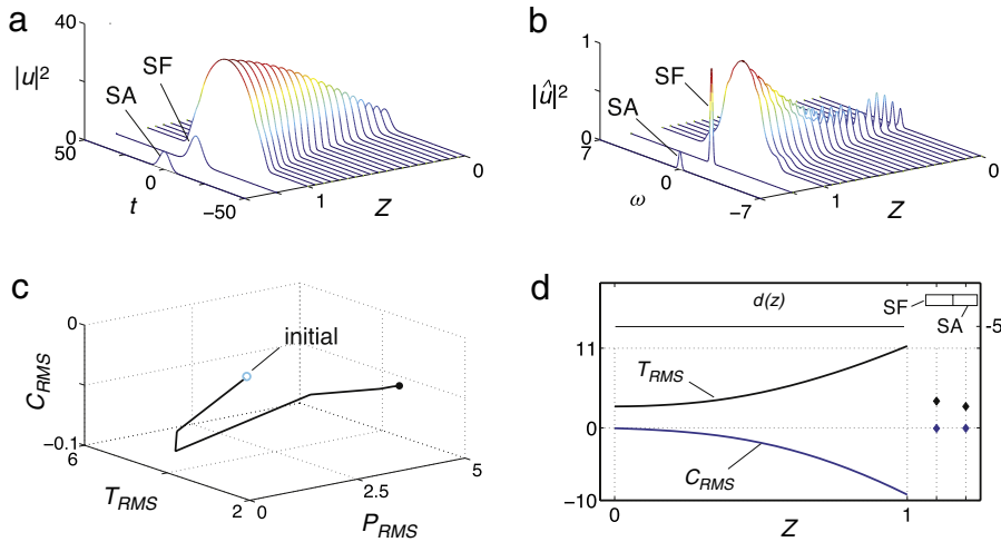
Fig. 26. (a) Temporal and (b) spectral evolution of the power per map period once steady state evolution is achieved from the solution to Eqs. (82)–(84) with discrete actions (92) and (94). Here F(x) = 0 , d_2 = -5 , l_1 = 0 , \epsilon = 1 , and dissipative parameters g_0 = 2.5 , l_0 = 0 , e_0 = 600 , \nu = 0 , q_0 = 0.8 , p_s = 3 , and \Omega_F = 0.3 . The spectral filter and saturable absorber follow the normal GVD segment. (c) Poincare map taken in the middle of the anomalous dispersion segment. (d) Intra-map evolutions of the RMS pulse duration and chirp parameter once steady state evolution is reached.
