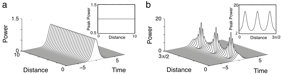
Fig. 1. (a) Fundamental soliton solution and (b) 2-soliton solution for the conservative NLSE (2) with g = 0 and s = d = 1 . Note that (a) represents a stationary solution and (b) represents a periodic breathing solution. This is highlighted in the insets which show the evolution of the peak power.
