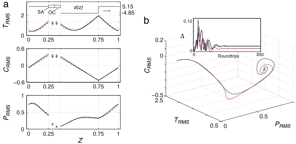
Fig. 24. (a) RMS pulse parameters over one map period once steady state evolution is achieved and (b) Poincare map taken at the point in the middle of the anomalous GVD segment from direct simulation of Eqs. (82)–(84) with discrete actions Eq. (92)–(93) (black) compared with that found from the reduced model equations (91) with discrete transfer functions Eq. (96)–(97) (red). Inset: absolute errors \Delta are shown for the RMS pulse parameters T_{RMS} (blue), P_{RMS} (red), and C_{RMS} (black). All parameters are the same as in Fig. 22. (For interpretation of the references to colour in this figure legend, the reader is referred to the web version of this article.)
