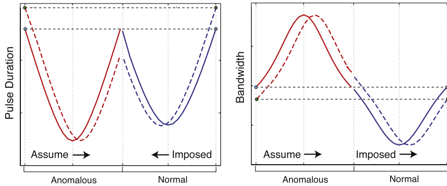
Fig. 7. Typical pulse duration and bandwidth for periodic DM soliton evolution (solid). Hypothetical evolution when it is assumed that CFP in the anomalous GVD segment is moved to the right of the centre of the anomalous GVD segment.
