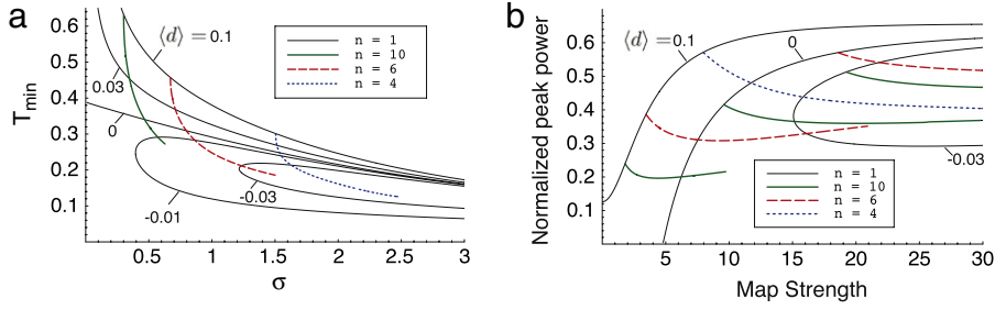
Fig. 10. Solution branches to the TM equations (50) for a lossless system ( c(z) = 1 ) with a two-step dispersion map (47). (a) Dependence of minimum T on the energy parameter \sigma = pN^2/d . Thin lines correspond to one-period solutions for various average dispersions and thick/dashed lines correspond to multiple-period solutions with \langle d \rangle = 0.1 . (b) Dependence of normalized power N_{\text{norm}}^2 on the map strength. Both one-period and multiple-period branches are shown for average dispersion values \langle d \rangle = 0.1, 0, -0.03 . Normalizations and map strength are the same as in Fig. 9.
