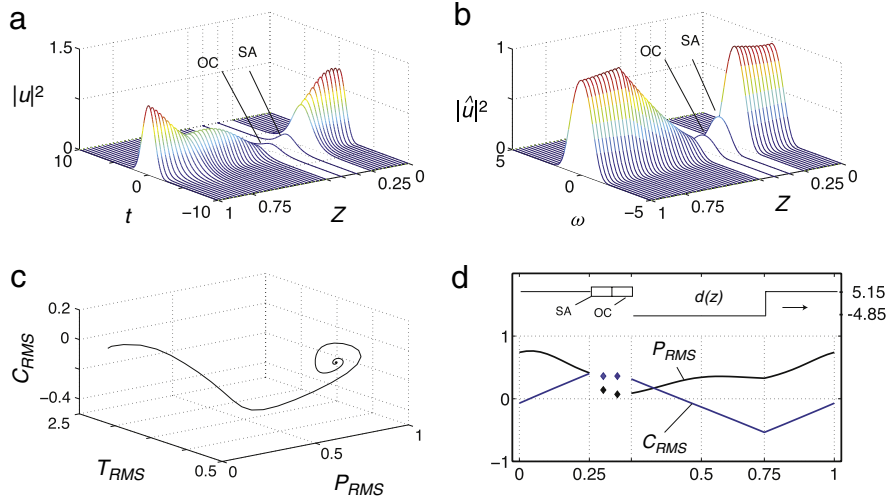
Fig. 22. (a) Temporal and (b) spectral evolution of the power per map period once steady state evolution is achieved from the solution to Eqs. (82)–(84) with discrete actions Eq. (92)–(93). Here F(x) = 0 , d = 5 , \langle d \rangle = 0.15 , \epsilon = 1 , and dissipative parameters g_0 = 0 in the anomalous GVD segment, g_0 = 4 in the normal GVD segment, l_0 = 0.1 , e_0 = 2 , v = 0.05 , q_0 = 0.5 , p_s = 3 , and R = 0.5 . The saturable absorber and output coupler are after the anomalous GVD segment. (c) Poincaré map taken in the middle of the anomalous dispersion segment. (d) Intra-map evolutions of the RMS pulse duration and chirp parameter once steady state evolution is reached.
