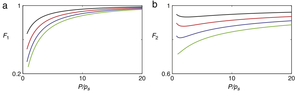
Fig. 23. (a) Peak power and (b) pulse duration response (96) of the discrete saturable absorber for q_0 = 0.3 (black), 0.5 (red), 0.7 (blue) and 0.9 (green). (For interpretation of the references to colour in this figure legend, the reader is referred to the web version of this article.)
