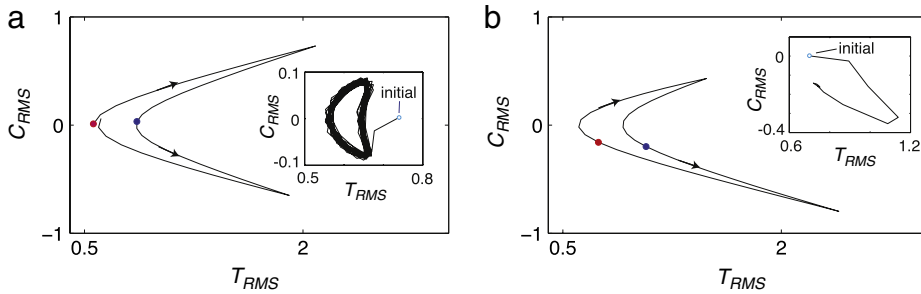
Fig. 18. Phase plane and Poincaré map (insets) taken at the middle of the anomalous GVD segment for the solutions obtained from Eqs. (82)–(84) with the same parameters as in Fig. 17 but with (a) F(x) = \nu = 0 and (b) F(x) = 1/(1+x) and \nu = 0.3 . The red (blue) dots on the phase plane correspond to the middle of the anomalous (normal) GVD segments. (For interpretation of the references to colour in this figure legend, the reader is referred to the web version of this article.)
