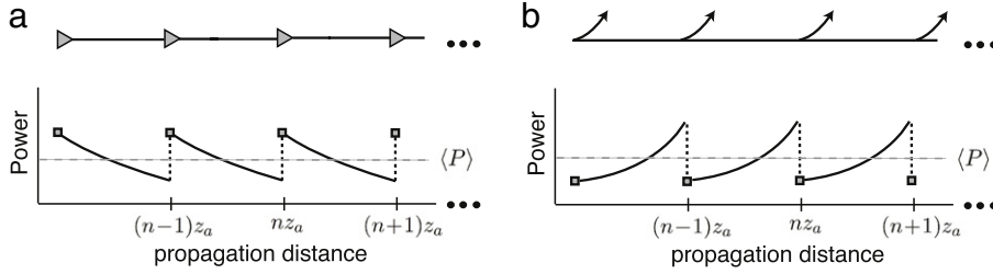
Fig. 2. Typical optical systems where dissipative elements are included along with dispersion compensation. The top panel shows schematically: (a) consecutive fibre spans and amplifiers (grey triangles); and (b) three round trips with periodic power out-coupling (out facing arrows) from a laser cavity. The value \langle P \rangle is the average power, and z_n is the length of the n th segment or round trip. (a) Example of a telecommunications system where the power is attenuated by fibre loss and regenerated by amplification. (b) Example of a laser application where the power is amplified by an active fibre and part of the signal is output at discrete points.
