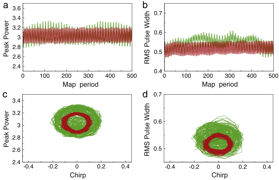
Fig. 8. Stroboscopic (taken at the middle of the anomalous GVD segment) evolution of (a) peak power and (b) RMS pulse width launched either at the CFP in the middle of the anomalous GVD fibre (red) or slightly from the CFP (green). Stroboscopic (taken at the middle of the anomalous GVD segment) evolution in the (c) power, chirp (d) width, chirp phase planes. (For interpretation of the references to colour in this figure legend, the reader is referred to the web version of this article.)
