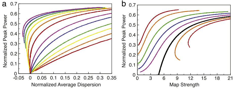
Fig. 9. Solution curves found from solving the TM equations (50). (a) Lines of constant map strength (right to left) S = 0.5, 1, 1.5, 2, 3, 4, 6, 8, 10, 12, 14, 16 . (b) Lines of constant average dispersion (right to left) ( d = -0.02, -0.01, 0.0, 0.02, 0.05, 0.1, 0.2, 0.3 ).
