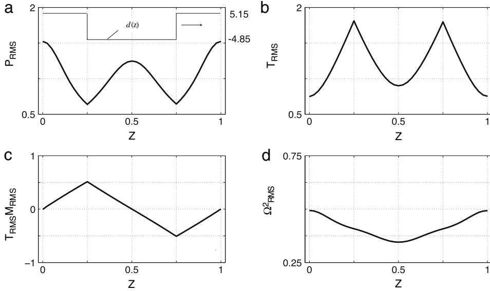
Fig. 4. The slow evolution of the RMS parameters for a typical piecewise constant dispersion map.
