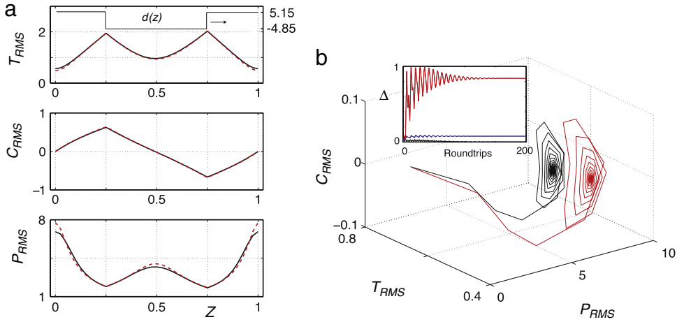
Fig. 21. (a) RMS pulse parameters over one map period once steady state evolution is achieved and (b) Poincaré map taken at the point in the middle of the anomalous GVD segment from direct simulation of Eqs. (82)–(84) (black) compared with that found from the reduced model equations (91) (red). Inset: the \Delta values are shown for the RMS pulse parameters T_{RMS} (blue), P_{RMS} (red), and C_{RMS} (black). All parameters are the same as in Fig. 17. (For interpretation of the references to colour in this figure legend, the reader is referred to the web version of this article.)
