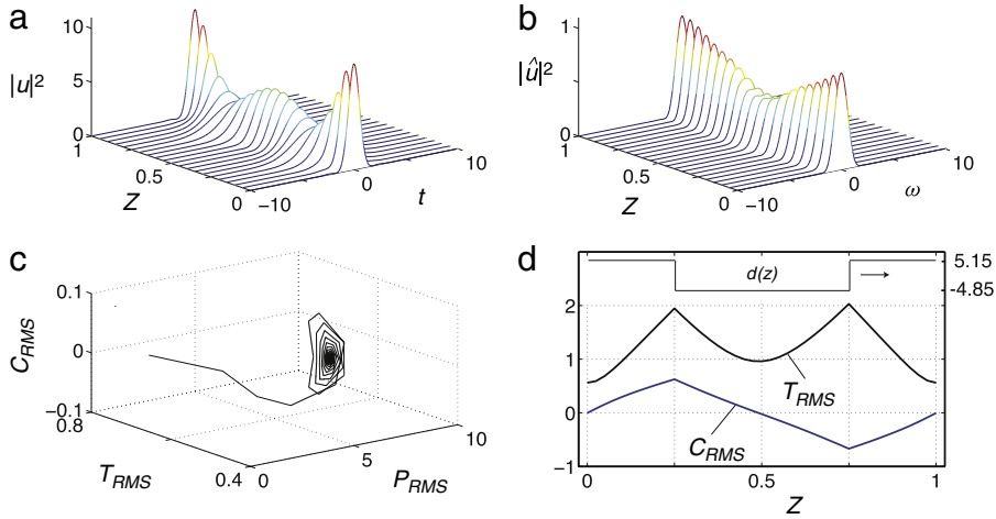
Fig. 17. (a) Temporal and (b) spectral evolution of the power per map period once steady state evolution is achieved from the solution to Eqs. (82)–(84) with d = 5 , \langle d \rangle = 0.15 , \epsilon = 1 , and dissipative parameters g_0 = l_0 = 0.7 , e_s = 2 , p_0 = 10 , and \nu = 0 . The nonlinear gain function is F(x) = 1/(1+x) . (c) Poincaré map taken in the middle of the anomalous dispersion segment. (d) Intra-map evolutions of the RMS pulse duration and chirp parameter once steady state evolution is reached.
