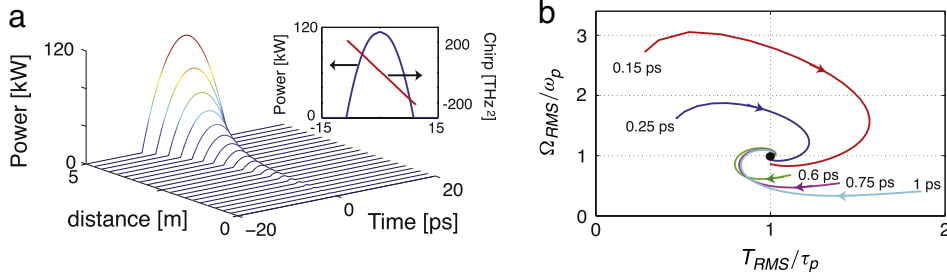
Fig. 16. (a) Solution from Eq. (75) with initial Gaussian pulse of energy 100 pJ and FWHM pulse duration 500 fs over 5 m of propagation. The parameters are \beta_2 = 0.025 \text{ ps}^2/\text{m} , \gamma = 0.005 \text{ 1/(W m)} , g = 0.95 \text{ 1/m} , \Gamma = \delta = 0 , and \Omega_f \rightarrow \infty . Inset: power and chirp profiles after 5 m propagation distance. (b) Phase portrait with normalized RMS pulse duration and bandwidth phase variables from similar numerical simulations as in (a), but with varying initial FWHM pulse durations ranging from 150 fs to 1 ps.
