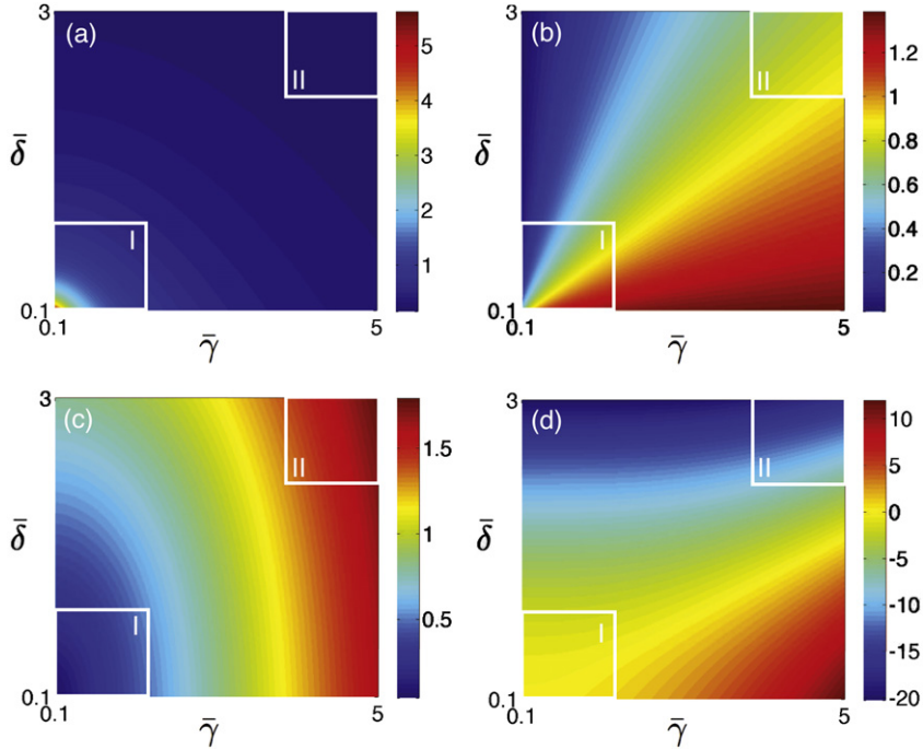
Fig. 14. Solution to the system (77) for (a) duration \tau/\tau_0 , (b) chirp parameter C , (c) bandwidth \mathcal{B} , and (d) gain parameter (g - \Gamma)\Omega_g^2\tau_0^2 with D = 0 .
